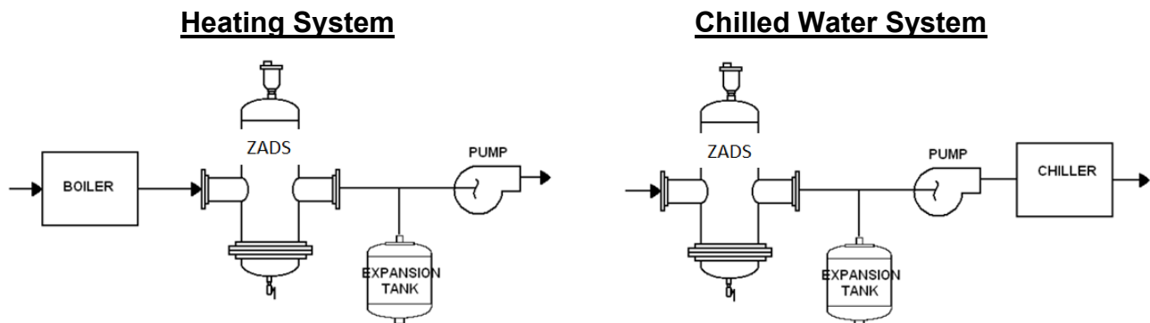
Figure 2: Suggested Mounting Locations
