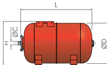
13-21 gallons Horizontal
