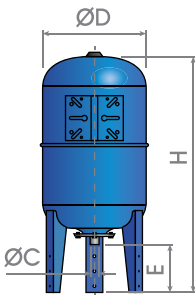
13-21 gallons Vertical
