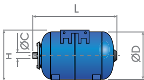
2-6 gallons Horizontal
