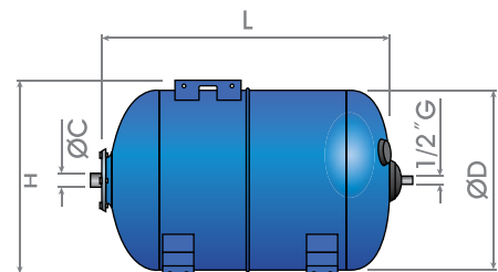
26-80 gallons Horizontal
