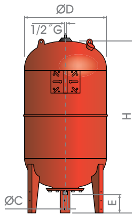
26-132 gallons Vertical
