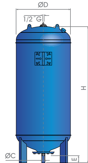
198-264 gallons Vertical
